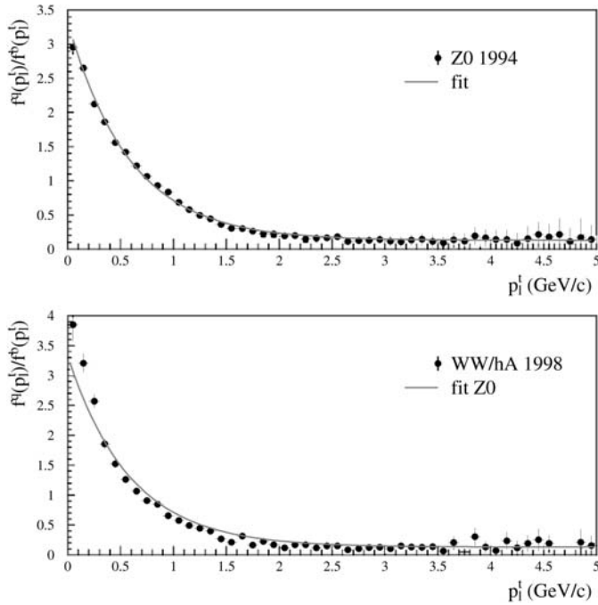
Fig. 18. The upper figure shows the ratio of the numbers of light-quark and b -quark events as a function of the lepton transverse momentum (dots), as extracted from simulated hadronic Z decays. The line is the fit to that ratio. The lower figure shows the same ratio, extracted from a simulated Higgs signal and WW background at LEP2. The line is the Z fit
