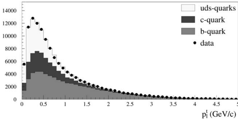
Fig. 16. Transverse momentum distribution of identified leptons with respect to the jet from which they originate, simulated in hadronic Z decays at LEP1. The contributions from light quarks, c -quarks and b -quarks are added and compared to the data
