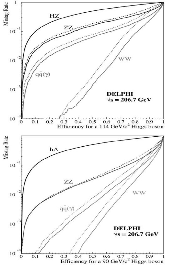
Fig. 26. Expected SM background mis-tag rates at \sqrt{s} = 206.7 GeV, as functions of the signal efficiency for a Standard Model Higgs boson of mass 114 \text{ GeV}/c^2 (top) and MSSM Higgs boson of mass 90 \text{ GeV}/c^2 and \tan \beta = 20 (bottom) when varying the cut on the equalised b -tagging variable (solid lines) and combined b -tagging variable (dotted lines)
