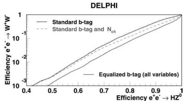
Fig. 20. Mis-tagging efficiency for e^+e^- \rightarrow W^+W^- versus e^+e^- \rightarrow HZ selection efficiency, as obtained from standard combined b -tagging, b -tagging equalised with respect to N_{\text{ch}} , and equalised b -tagging with the complete set of variables (see text for details)
