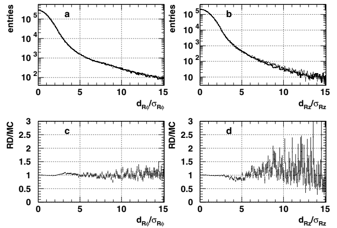
Fig. 12. a,b The R\phi and Rz significance distributions for tracks with negative IP after the tuning procedure. The points with errors are real data, the histogram is simulation. c,d The ratios of these distributions (data divided by simulation). The improvement resulting from tuning is clearly visible (cf. Fig. 11)
