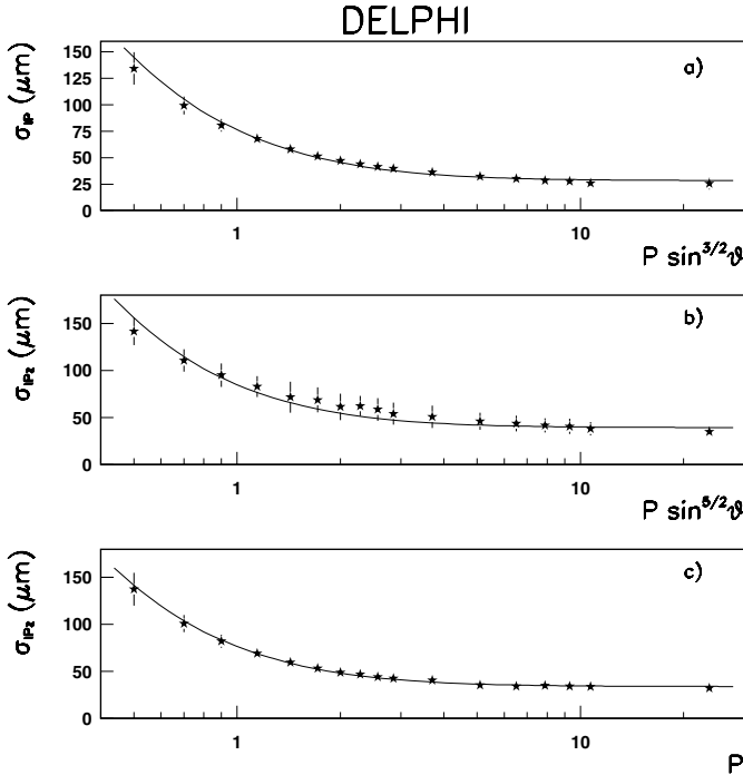
Fig. 4. The R\phi IP uncertainty as a function of p \sin^{3/2}\theta (upper plot), the Rz IP uncertainty as a function of p \sin^{5/2}\theta (middle plot) and the Rz IP uncertainty as a function of p for tracks with \theta = [80^\circ : 100^\circ] , i.e. perpendicular to the beam direction (lower plot). The data are from the Double Sided Vertex Detector at the Z. The curves are parameterisations of a constant intrinsic resolution term and a momentum-dependent multiple scattering contribution. Momenta are in \text{Gev}/c
