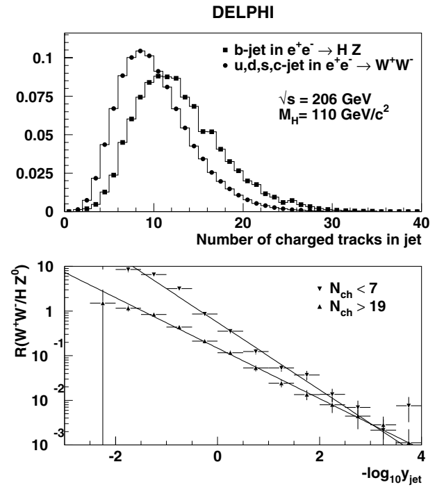
Fig. 19. Upper plot: Simulated distributions of the number of tracks in a b -jet from the e^+e^- \rightarrow HZ process and in a light quark jet from the e^+e^- \rightarrow W^+W^- process. Lower plot: the ratio R(W^+W^-/HZ) of the number of light quark jets from the e^+e^- \rightarrow W^+W^- process to that of b -jets from e^+e^- \rightarrow HZ process in the simulation (arbitrary normalisation) as a function of -\log_{10} y_{\text{jet}} , shown separately for jets with less than 7 or greater than 19 tracks. The lines in each case show the exponential fit of these rates
