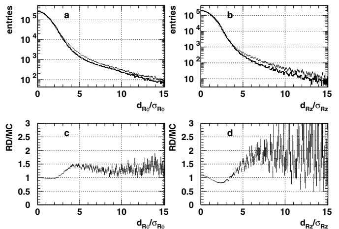
Fig. 11. a,b The R\phi and Rz significance distributions for tracks with negative IP. The points with errors are real data, the histogram is simulation. c,d The ratios of these distributions (data divided by simulation)
