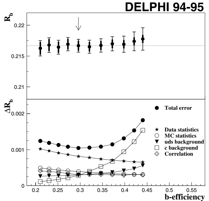
Fig. 22. Stability of the R_b result as a function of the b -tagging efficiency, for data collected in 1994–5. The arrow shows the b -efficiency chosen for the final result
