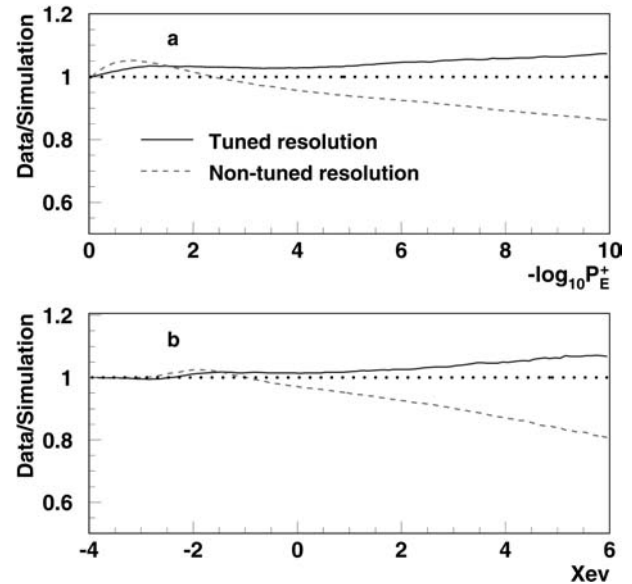
Fig. 13a,b. The integrated data to simulation ratio of the fraction of selected hemispheres as a function of the cut on the b -tagging variable for a the lifetime tagging variable P_E^+ , calculated using all positive lifetime IP tracks in an event (see Sect. 3.5) and b combined tagging variable X_{ev} (see Sect. 4), with tuned (full line) and non-tuned (dashed line) track resolution
