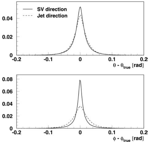
Fig. 6. Distributions of the difference between reconstructed and generated directions of b -hadrons for events with a reconstructed secondary vertex, for simulated Z events. The B direction is defined as the direction from the primary to the secondary vertex (solid line) or as the jet direction (dashed line). Especially in \phi , the definition using the secondary vertex gives a better description of the B direction
