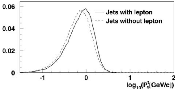
Fig. 17. Distribution of \log_{10}(P_s^t) for jets with (solid line) and without (dashed line) leptons
