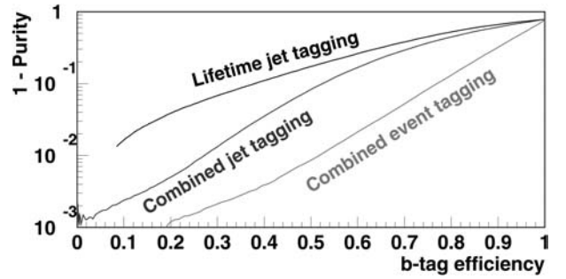
Fig. 15. Background suppression in Z hadronic events using combined b -tagging
