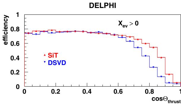
Fig. 3. Selection efficiency of Z \rightarrow b\bar{b} events versus \cos \Theta_{\text{thrust}} using the combined event b -tagging variable X_{\text{ev}} > 0 for the Silicon Tracker and the Double Sided Vertex Detector. ( X_{\text{ev}} is defined in Sect. 4.1.) The extra coverage provided by the Silicon Tracker in the forward direction is clearly visible
