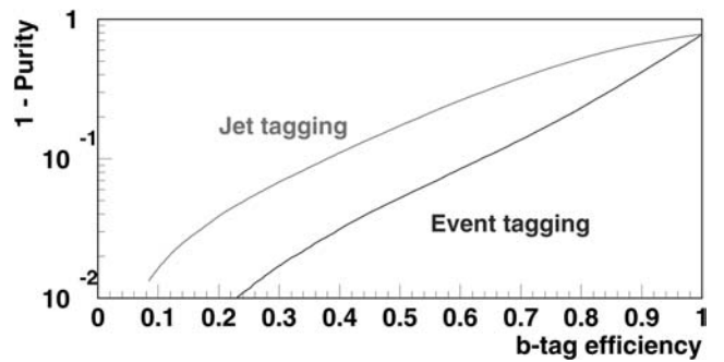
Fig. 10. Background suppression in simulated Z hadronic events using lifetime tagging. The efficiency is the fraction of b -jets that are tagged as coming from b -quarks, while the purity is the fraction of b -tags that are really from b -quarks
