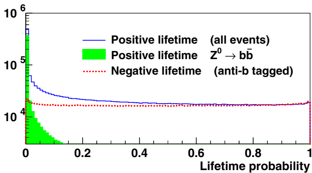
Fig. 9. Distributions of positive and negative lifetime probabilities ( P_N^+ and P_N^- respectively) for simulated Z hadronic events
