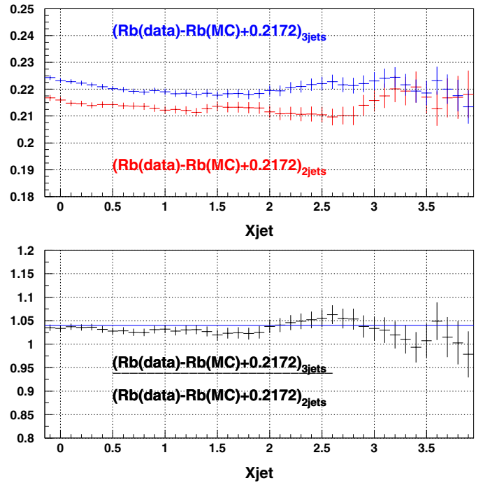
Fig. 21. Comparison of the measurements of the R_b ratio in 2 and 3 jet events at the Z , as a function of the cut in the b -tagging variable X_{\text{jet}} . The simulation used JETSET 7.4
