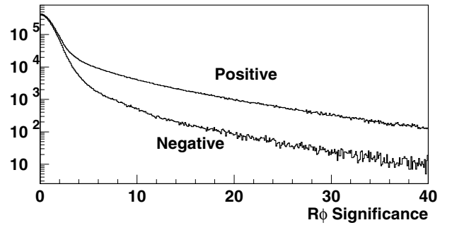
Fig. 7. Distributions of positive and negative R\phi significances and data for Z hadronic decays. The excess of tracks with large positive significance is due to long-lived particles
