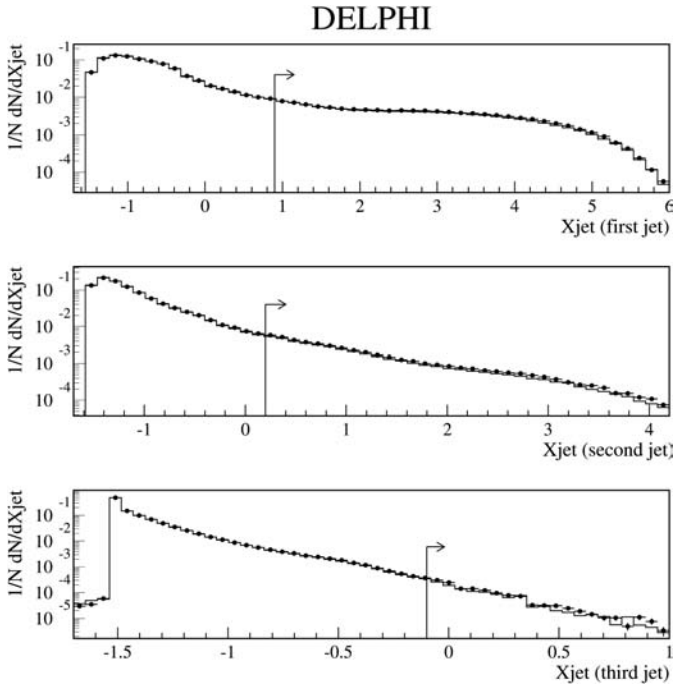
Fig. 23. Distribution of the b -tagging variables for the first three jets, ordered according to their b -tagging variable, for Z data (dots) and simulation (histogram). The arrows show the positions of the cuts used to select the b jets. The figure is from [22]
