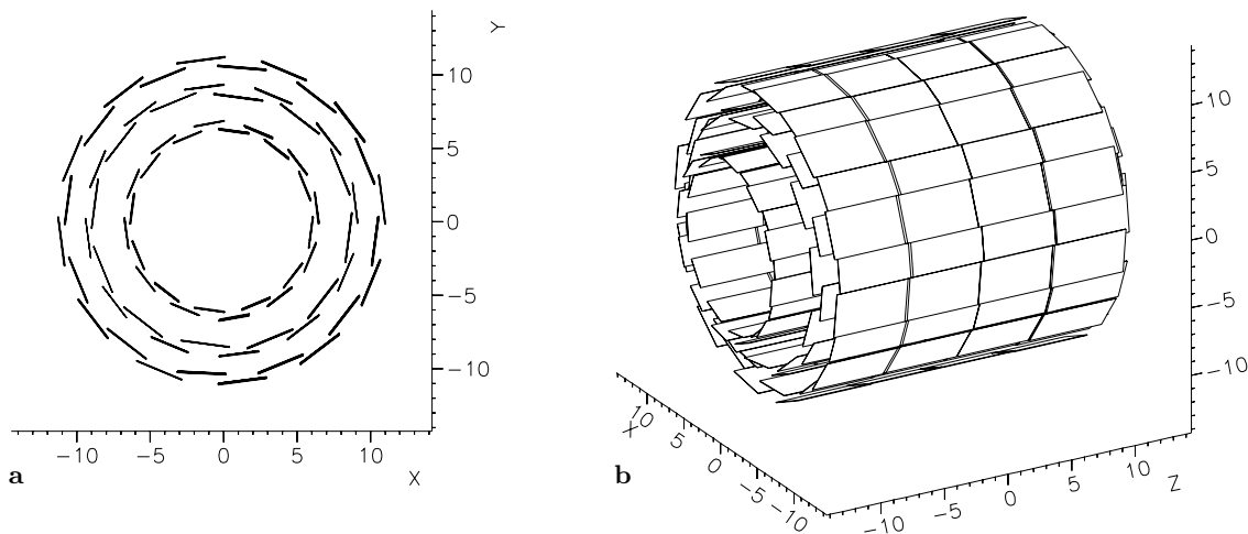
Fig. 1a,b. Schematic cross sections of the Double Sided Vertex Detector in a the transverse ( R\phi ) view and b a three-dimensional view. Dimensions are in cm
