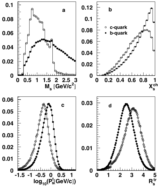
Fig. 14a–d. Distributions of discriminating variables for b - and c -quark jets for simulated Z hadronic events. a Mass of particles in SV. b Fraction of charged jet energy included in SV. c Transverse momentum at SV. d Rapidity for each SV track
