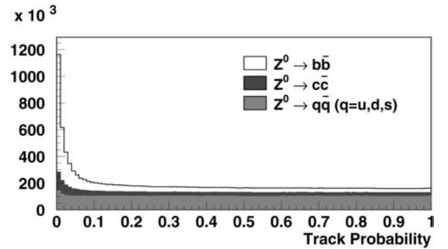
Fig. 8. Simulated distributions at the Z of the R\phi track IP probabilities for different quark flavours, for tracks with positive lifetime-sign IPs
