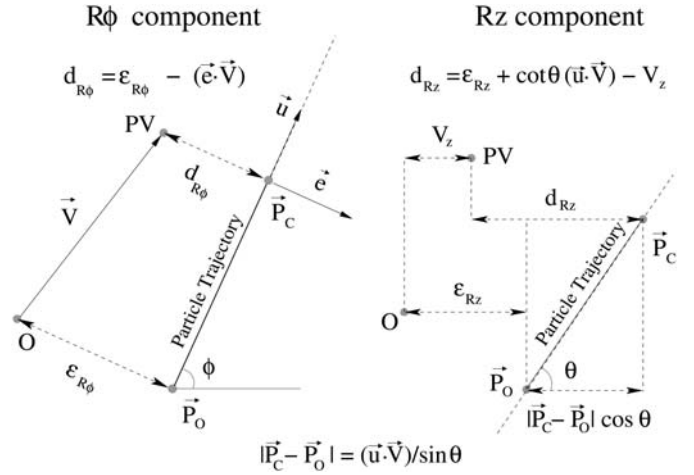
Fig. 5. Definition of R\phi and Rz IP components. \vec{u} is a unit vector along the R - \phi projection of the track direction, and \vec{e} is another unit vector in the R\phi plane, perpendicular to \vec{u} . \vec{V} is a vector from the origin O to the primary vertex PV. P_0 and P_C are the points of closest approach in the R\phi plane of the track trajectory to O and to PV respectively. The diagrams show the projections onto the R\phi and Rz planes. The IP components are d_{R\phi} and d_{Rz} , while \varepsilon_{R\phi} and \varepsilon_{Rz} are the corresponding components from P_0 to the origin
