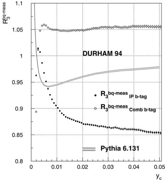
Fig. 24. The R_3^{bq-meas} observable from simulated DELPHI data for the two tagging techniques and the parton level R_3^{bq-part} obtained with PYTHIA 6.131. The DURHAM jet finding algorithm is used with a cut on the jet resolution parameter at y_c
