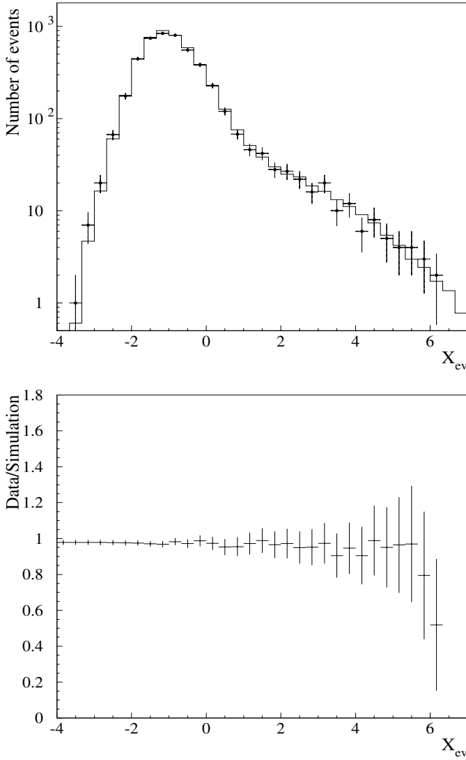
Fig. 25. Top: distribution of the equalised b -tagging variable for 4-jet events at \sqrt{s} = 192\text{--}210 GeV, data (dots) and simulation (solid line). Bottom: ratio of the integrated tagging rates in data and simulation as a function of the cut in the equalised b -tagging variable. The agreement between data and simulation is satisfactory
